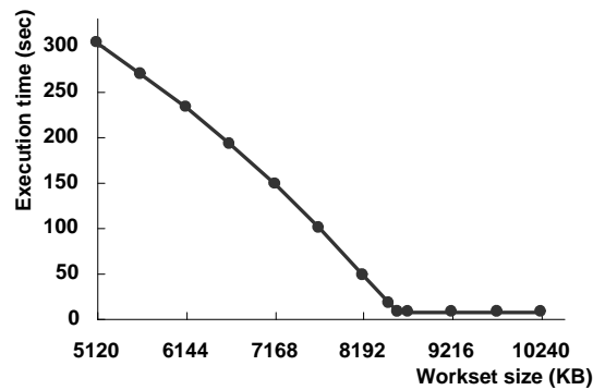
Figure 11: Control of memory usage on Linux.
