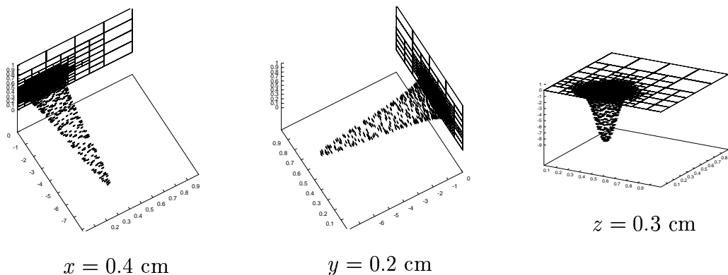
Fig. 4.1: Final triangulation
