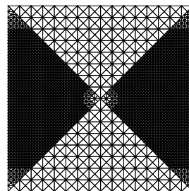
Fig. 4.2b: Discontinuous coefficient
