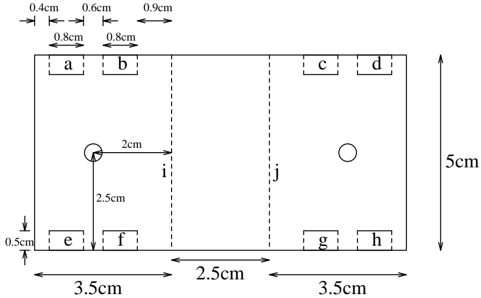
Figure 15: Base plate
