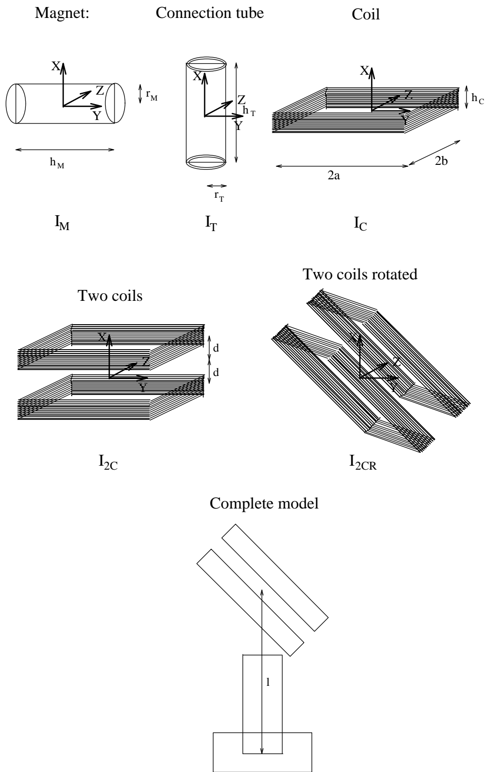
Figure 1: Inertia tensor model
