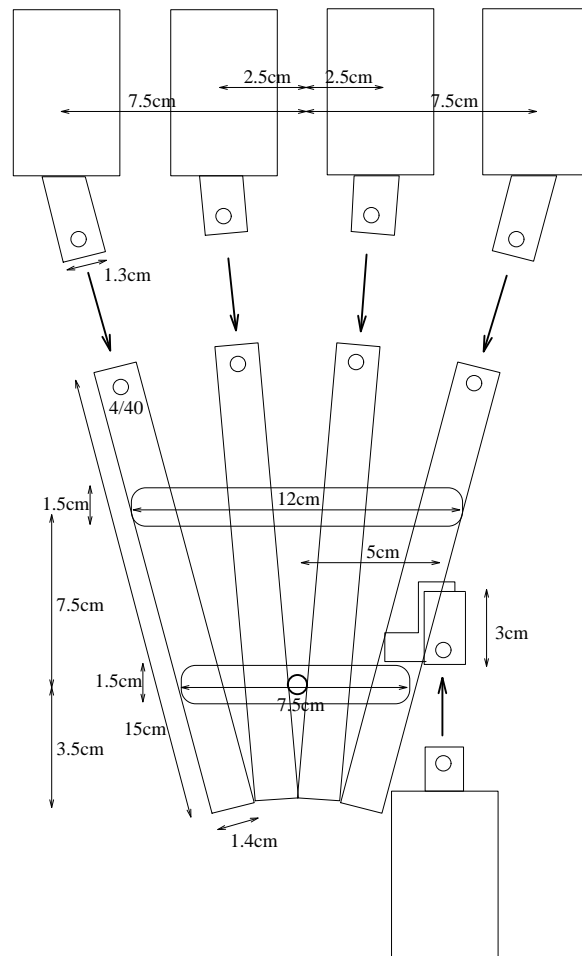
Figure 21: Hand assembly
