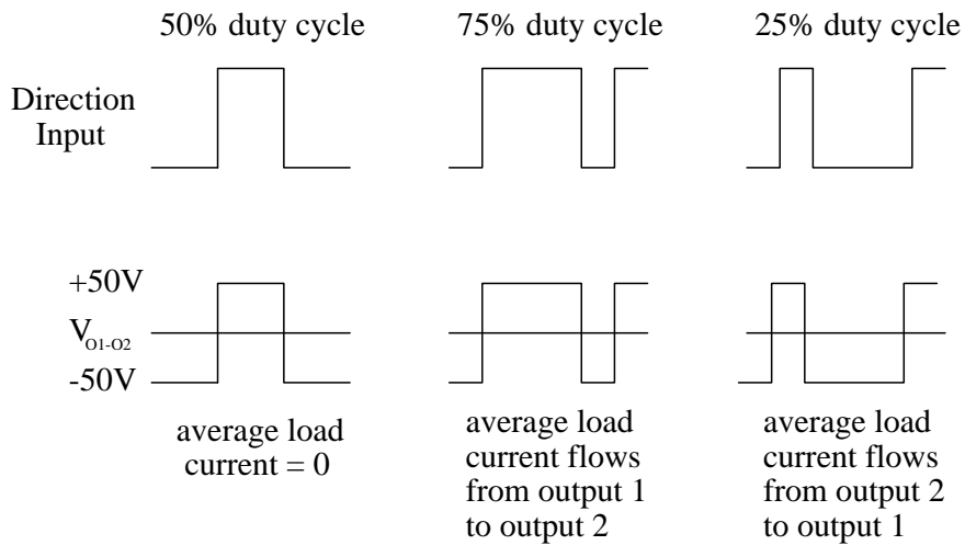
Figure 27: LMD 18201 3A, 55V, H-Bridge
