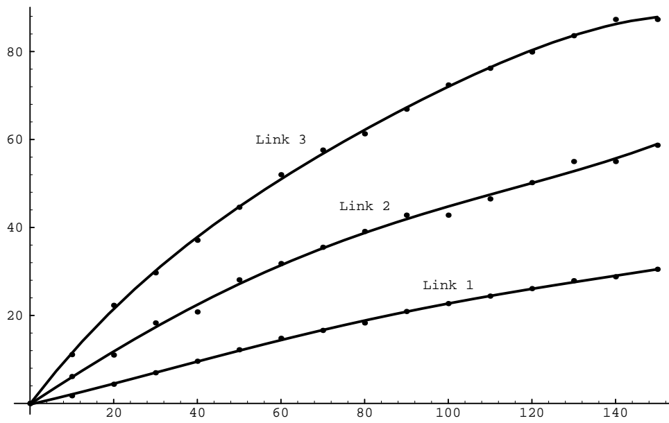
Figure 11: Temperature over time for U=20V \Delta T[K](t[s])
