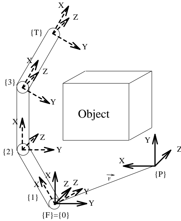
Figure 23: Frame definitions
