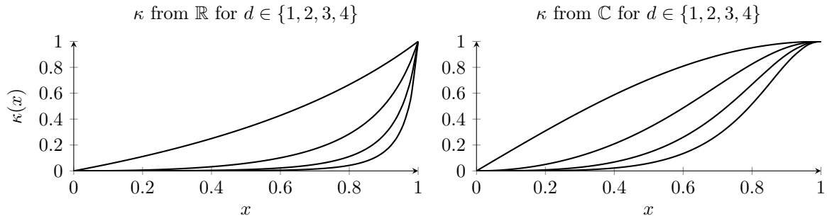
Figure 3: Examples of specific functions \kappa for d = 1, 2, 3 , and 4 from the analysis in Section 4. Higher values of d tend closer to the x -axis for longer. Observe how \kappa over \mathbb{C} is higher than over \mathbb{R} for identical d , indicating that, all else equal, the protocol has better (lower) soundness error when instantiated over \mathbb{C} .
