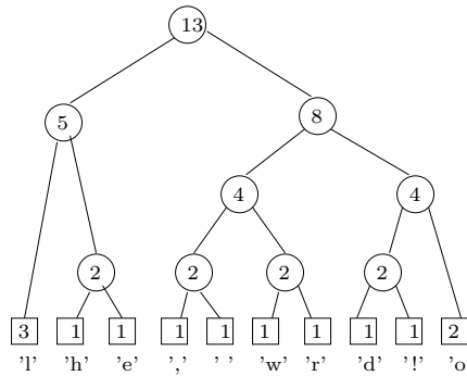
Figure 1: Huffman code for “Hello, world!”
