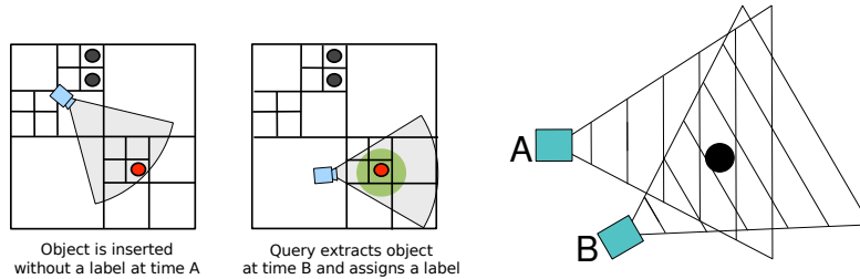
Figure 5: Temporal label propagation. At position/time A , the robot can see the black object, but the object is out of stereo range, so it cannot be labeled. It is inserted into the quad-tree. At position/time B , the object is seen from a different, closer view and a stereo label is obtained. Now the view of the object from position A can be extracted from the quad-tree and trained on using the label from position B .
