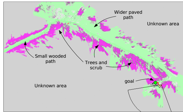
Figure 9: This is a global map produced by the robot while navigating toward a goal (green circle). The robot sees and follows the path and resists the shorter yet non-traversable direct path through the woods.
