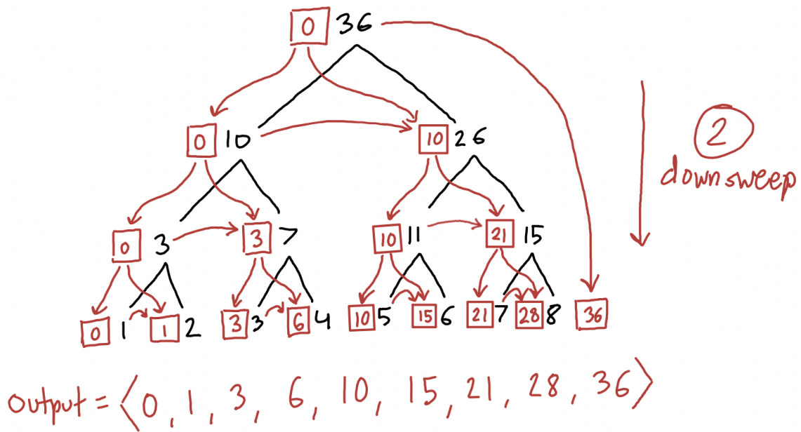
Figure 1: Upsweep-downsweep prefix sums
