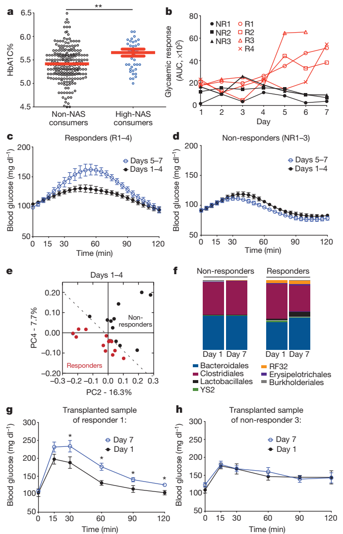
Figure 4 | Acute saccharin consumption impairs glycaemic control in humans by inducing dysbiosis. a , HbA1C% of high NAS consumers ( N = 40 ) versus non-consumers ( N = 236 ). ^{**} Rank sum P value < 0.002 . b , Daily incremental area under the curve (iAUC) of OGTT in 4 responders (R) and 3 non-responders (NR). c , d , OGTT of days 1–4 versus days 5–7 in 4 responders (c) or 3 non-responders (d). e , PCoA of 16S rRNA sequences from responders ( N samples = 16) versus non-responders ( N = 9 ) during days 1–4. f , Order-level relative abundance of taxa samples from days 1 and 7 of responders and non-responders. g , h , OGTT in germ-free mice ( N = 6 ) 6 days following faecal transplantation of D1 or D7 samples of responder 1 (R1, g ) or non-responder 3 (NR3, h ). Symbols, means; error bars, s.e.m. ^{*}P < 0.05 , ^{**}P < 0.01 , ANOVA and Bonferroni post hoc analysis.
