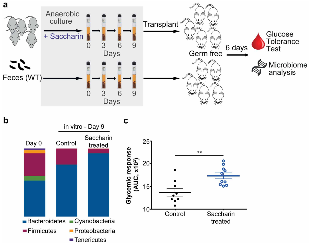
Extended Data Figure 8 | Saccharin directly modulates the microbiota. a , Experimental schematic. b , Relative taxonomic abundance of anaerobically cultured microbiota. c , AUC of germ-free mice 6 days following transplantation
