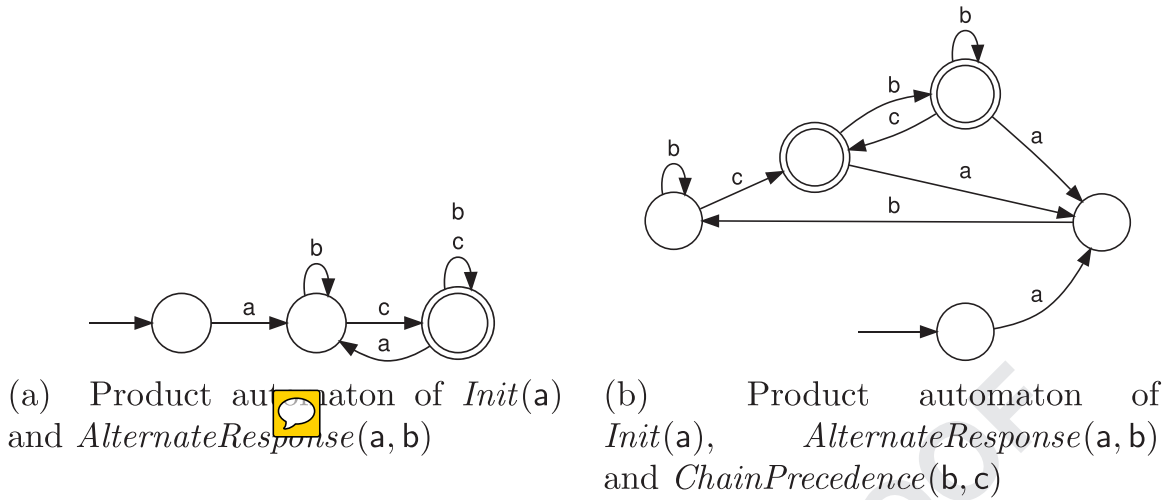
Fig. 4. Product automata of the FSAs shown in Fig. 3.
