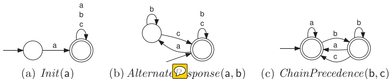
Fig. 3. FSAs accepting the traces compliant with some Declare constraints over the log alphabet \{a, b, c\} .
