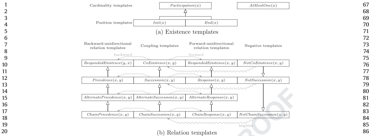
Fig. 1. The subsumption map of DECLARE templates. Templates are indicated by solid boxes. The subsumption relation is depicted as a line starting from the subsumed template and ending in the subsuming one, with an empty triangular arrow recalling the UML IS-A graphical notation. The coupling constraint templates are linked to the related forward-unidirectional relation constraint and backward-unidirectional relation constraint templates by means of grey arcs. The negative constraint templates are graphically linked to the corresponding coupling constraint templates by means of wavy grey arcs.
