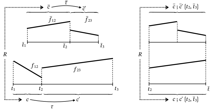
Fig. 4. Asynchronous hybrid simulation
