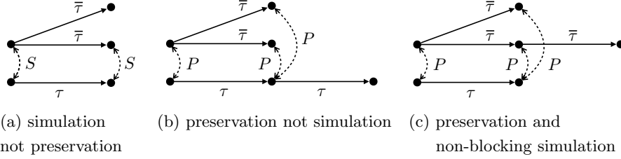
Fig. 11. Simulation versus preservation
