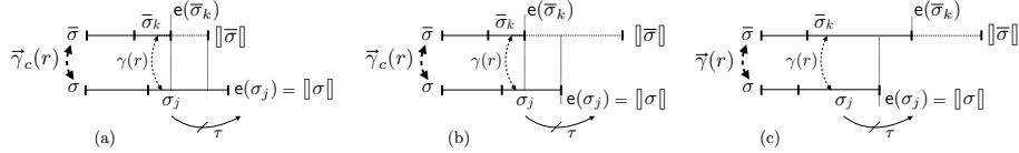
Fig. 12. Termination of concrete versus abstract trajectories
