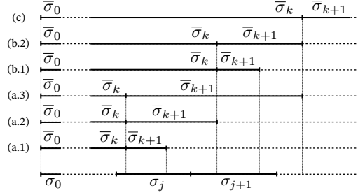
Fig. 13. Possible transition steps
