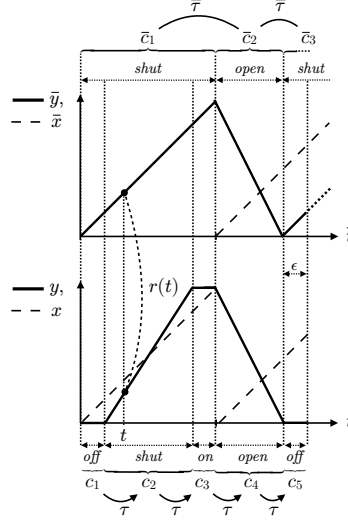
Fig. 14. Concrete and abstract transitions for the tank
