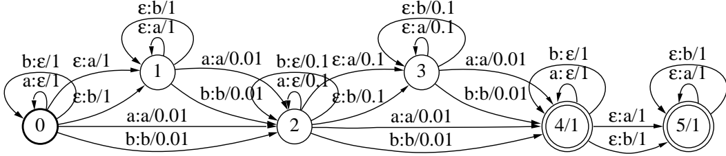
Figure 1: Gappy bigram rational kernel with decay factor \lambda = .1 . Bold face circles represent initial states and double circles indicate final states. Inside each circle, the first number indicates the state number, the second, at final states only, the value of the final weight function \rho at that state. Arrows represent transitions. They are labeled with an input and an output symbol separated by a colon and followed by their corresponding weight after the slash symbol.
