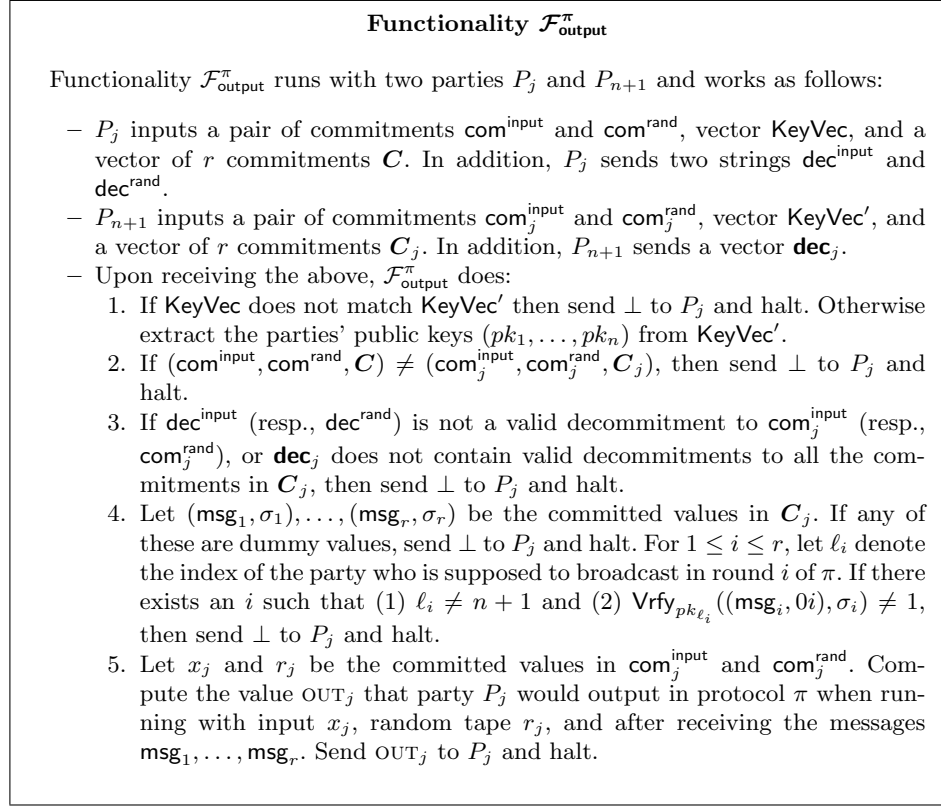
Fig. 2. The functionality computing the output of \pi
