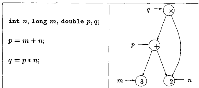
Figure 1: (a) Program Fragment. (b) Expression dags for p, q .
