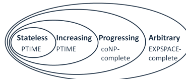
Fig. 1: Middlebox hierarchy.
