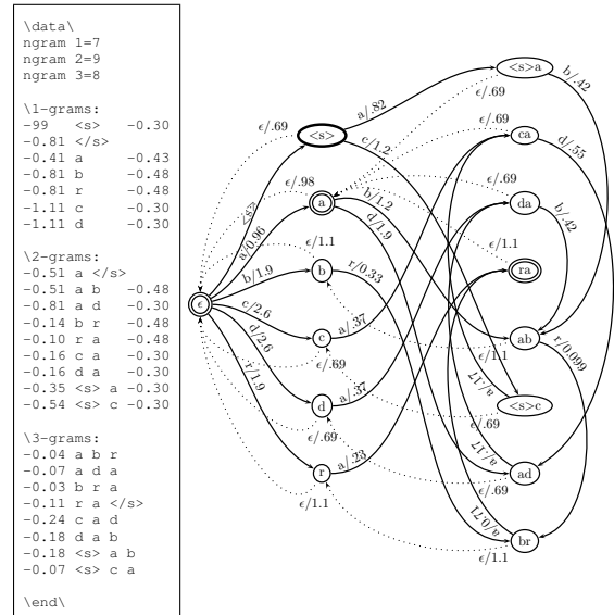
Figure 2: A trivial, but complete, trigram language model
