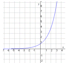
exponential function
