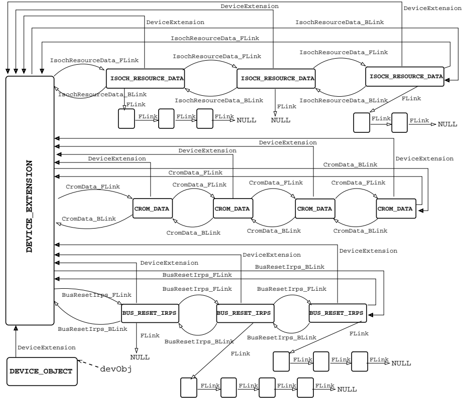
Fig. 1. Device driver-like heap configuration.
