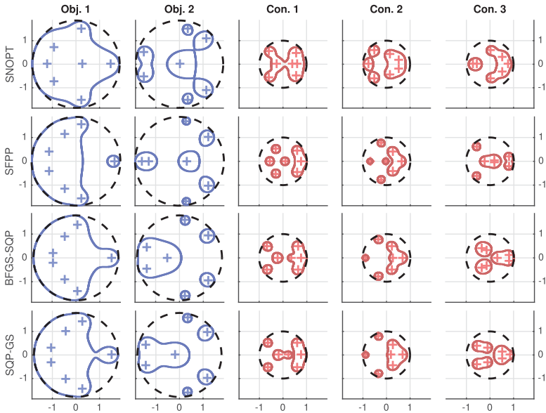
Figure A8. The four rows show the final pseudospectral configurations for the four controllers found by SNOPT, SFPP, BFGS-SQP, and SQP-GS (top to bottom) for the problem described in Figure A7. The left two columns indicate the plants in the objective while the right three columns indicate the plants in the constraint, with the plus signs indicating the eigenvalues. On the objective plots, the dashed black circle corresponds to the max pseudospectral radius of the two plants in the objective for that particular algorithm’s controller. The dashed black circle on the plots for constraints is the unit circle (the stability boundary). The solid lighter circles indicate the pseudospectral boundaries of each plant.
