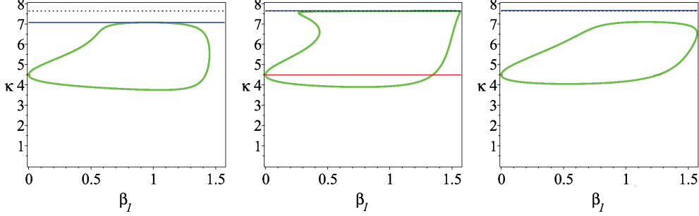
Fig. 8 Stability diagrams for (left) \alpha_1 = \alpha_1^* - 0.1 , (center) \alpha_1 = \alpha_1^* \approx 0.5885275986 and (right) \alpha_1 = \alpha_1^* + 0.1 . The green and blue curves respectively show the flutter and divergence boundaries. In the left and center panels, the critical load reaches the divergence boundary, but this is higher in the center panel, and there it is reached only if \beta_1 = \pi/2 . In the right panel, the flutter boundary prevents the critical load from reaching the divergence boundary.
