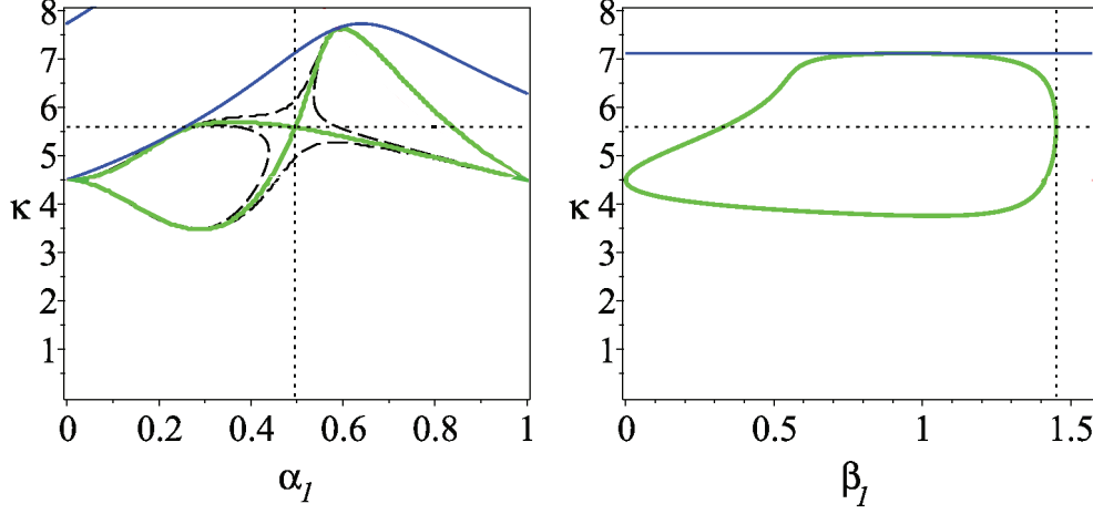
Fig. 4 Stability diagrams for (left) \beta_1 = \hat{\beta} = 1.450234089 in the (\alpha_1, \kappa) -plane and (right) for \alpha_1 = \hat{\alpha} = 0.4947347666 in the (\beta_1, \kappa) -plane. The solid blue curves designate the divergence boundary (3.3) and the solid green curves mark the flutter boundary (3.4). The flutter boundary in the left panel has a crossing at the saddle point located at \alpha_1 = \hat{\alpha} and \kappa = 5.591633160 . The black dashed curves in the left panel correspond to the flutter boundaries at (upper and lower curves) \beta_1 = \hat{\beta} - 0.01 and (left and right curves) \beta_1 = \hat{\beta} + 0.01 . In the right panel, the divergence boundary is a horizontal blue line with height \kappa = \hat{\kappa} = 7.113918994 .
