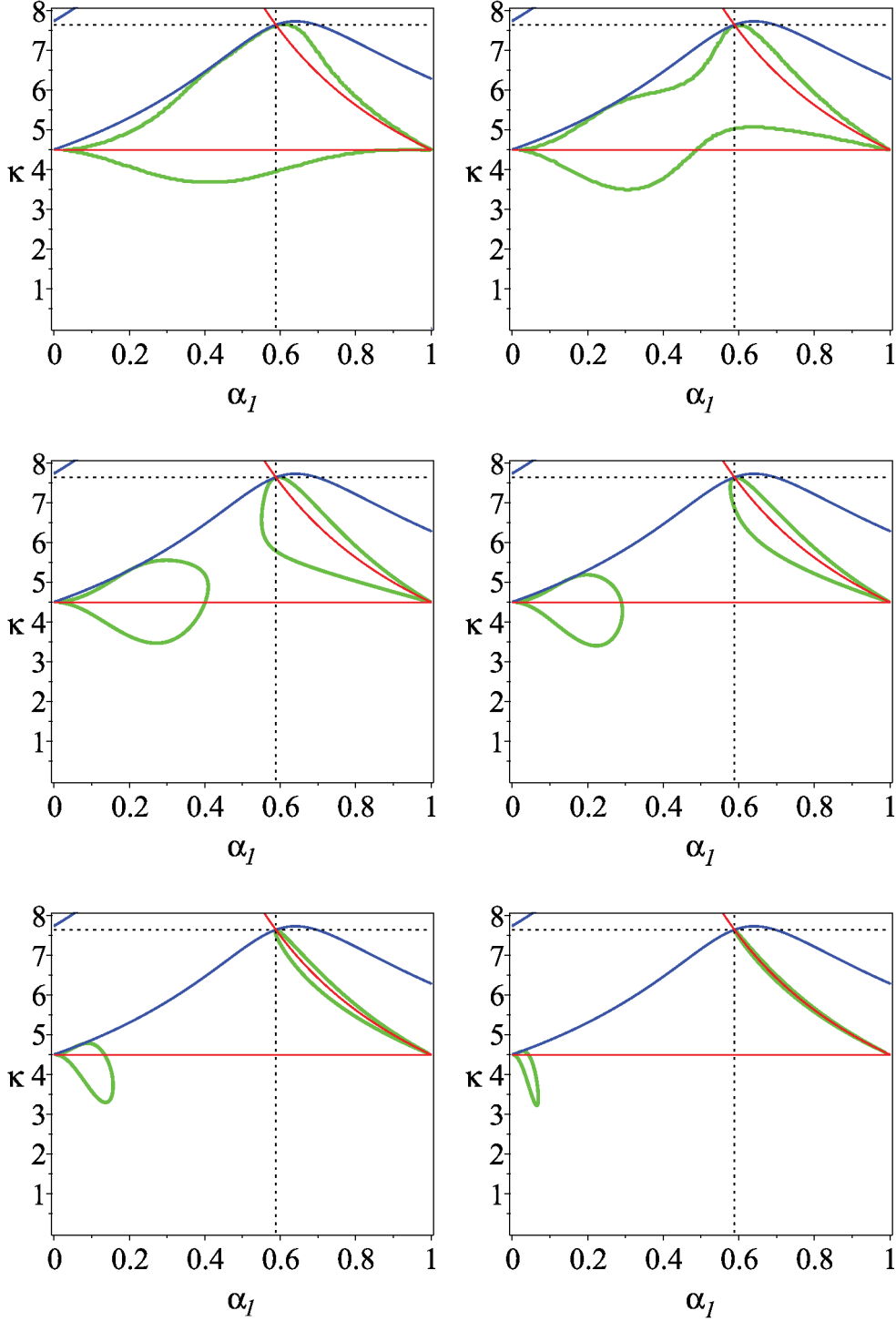
Fig. 7 Stability diagrams in the (\alpha_I, \kappa) -plane for (upper left) \beta_1 = \pi/2 - 0.5 , (upper right) \beta_1 = \pi/2 - 0.15 , (middle left) \beta_1 = \pi/2 - 0.1 , (middle right) \beta_1 = \pi/2 - 0.05 , (lower left) \beta_1 = \pi/2 - 0.01 , and (lower right) \beta_1 = \pi/2 - 0.001 . The black dashed lines intersect at the point with the coordinates of the optimal solution: \alpha_1^* \approx 0.588527598 and \kappa^* \approx 7.635002111 .
