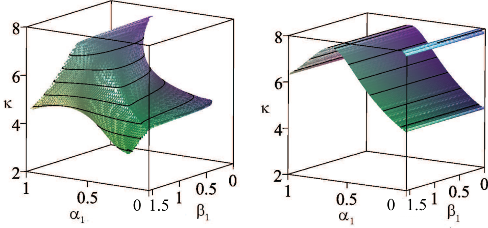
Fig. 3 The case of n = 2 concentrated masses. (Left) the flutter domain is a finite solid set in the (\alpha_1, \beta_1, \kappa) space, enclosed within the singular surface defined by (3.4). (Right) The divergence domain lies above the boundary set defined by (3.3). For a given (\alpha_1, \beta_1) , the critical value of the load parameter, \kappa_{\text{crit}}^{\alpha_1, \beta_1} , is the minimal value of \kappa that satisfies either (3.4) or (3.3), as this is the length of the longest vertical line segment rising from the point (\alpha_1, \beta_1, 0) that does not enter either the flutter or divergence domain. Consequently, this is the largest value \tilde{\kappa} such that the column is stable for all \kappa \in [0, \tilde{\kappa}) . The strongest stable column is obtained by finding (\alpha_1, \beta_1) with the largest possible critical load \kappa_{\text{crit}}^{\alpha_1, \beta_1} .
