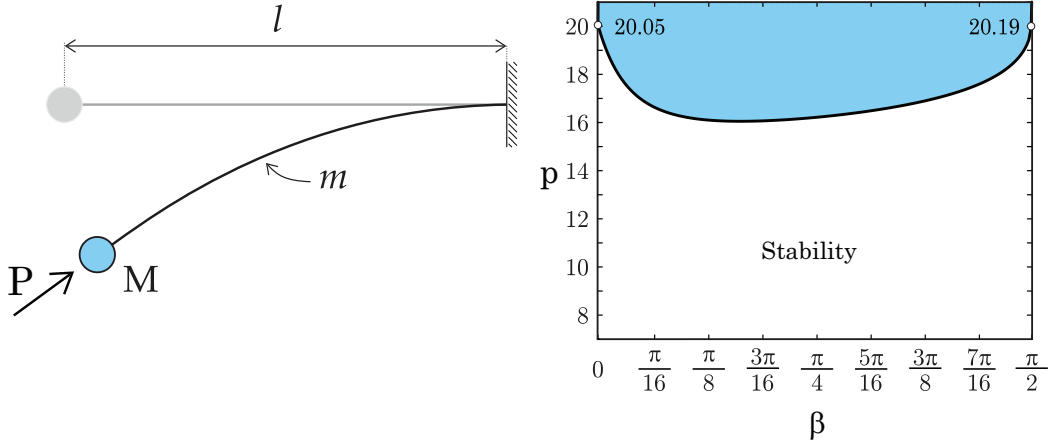
Fig. 1 The Pflüger column and its stability diagram. The ratio of the end mass to the mass of the column, \mu = M/(ml) , is parameterized by \mu = \tan \beta . The Beck column corresponds to the vanishing end mass ( M = 0 , so \beta = 0 ) and the weightless Pflüger column (or Dzhanelidze's column (6)) to the vanishing mass of the rod ( m = 0 , so \beta = \pi/2 ). The vertical axis of the stability diagram shows the dimensionless load (see (1.4)).
