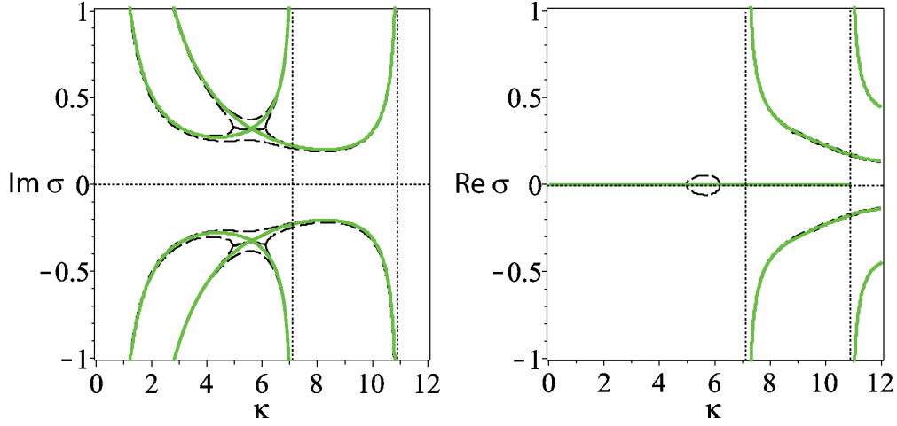
Fig. 5 (Left) imaginary and (right) real roots of the characteristic polynomial (3.2) for \alpha_1 = \hat{\alpha} = 0.4947347666 and (green, solid) \beta_1 = \hat{\beta} = 1.450234089 and (black, dashed) \hat{\beta} \pm 0.01 . A bubble of complex eigenvalues appears for \beta_1 = 1.450234089 - 0.01 and corresponds to flutter instability. The black dotted vertical line at \kappa = \hat{\kappa} = 7.113918994 is the onset of divergence instability. Increase in \beta_1 from \hat{\beta} - 0.01 to \hat{\beta} + 0.01 results in the disappearance of the complex eigenvalues and hence is accompanied by the transition from the overlapping eigenvalue branches to an avoided crossing that yields a jump in the critical load parameter to the maximal value that is reached at \kappa = \hat{\kappa} on the divergence boundary (56); see also the right panel of Fig. 4.
