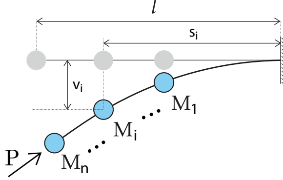
Fig. 2 The weightless ( m = 0 ) Beck column loaded by the follower force P with n concentrated masses ( M_1, M_2, \dots, M_i, \dots, M_n ) attached (52, 56).
