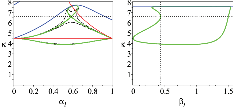
Fig. 6 Stability diagrams for (left) \beta_1 = \tilde{\beta} = 0.4342999969 in the (\alpha_1, \kappa) -plane and (right) for \alpha_1 = \tilde{\alpha} = 0.5810701268 in the (\beta_1, \kappa) -plane. The solid blue curves designate the divergence boundary (3.3), and the solid green curves mark the flutter boundary (3.4). The flutter boundary in the left panel has a crossing at the saddle point located at \alpha_1 = \tilde{\alpha} and \kappa = 6.600674669 . The black dashed curves in the left panel correspond to the flutter boundaries at (upper and lower curves) \beta_1 = \tilde{\beta} - 0.05 and (left and right curves) \beta_1 = \tilde{\beta} + 0.05 . In the right panel, the divergence boundary is the horizontal blue line with height \kappa = 7.607584259 . The horizontal red line shows the value \kappa_0 = 4.493409458 , which is the root of (3.5): the flutter boundary for the case \beta_1 = 0 . The other red solid curve in the left panel is the solution to (3.6): the flutter boundary for the case \beta_1 = \pi/2 .
