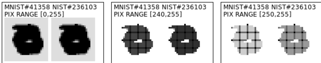
Figure 2.3: We have reproduced a defect of the original resampling code that creates low amplitude periodic patterns in the dark areas of thick characters.
