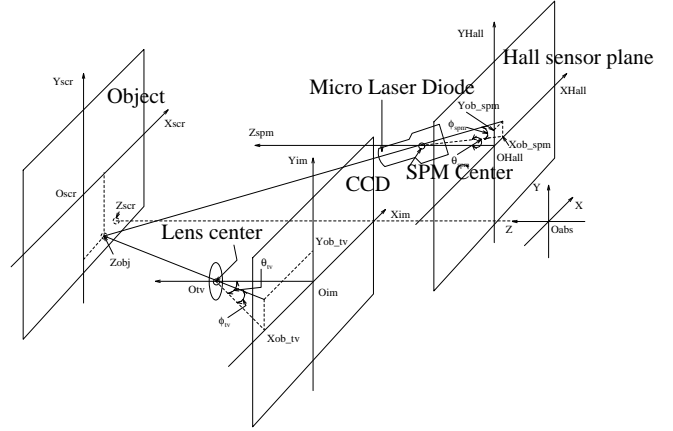
Figure 3: Coordinate frames used in triangulation calculations.
