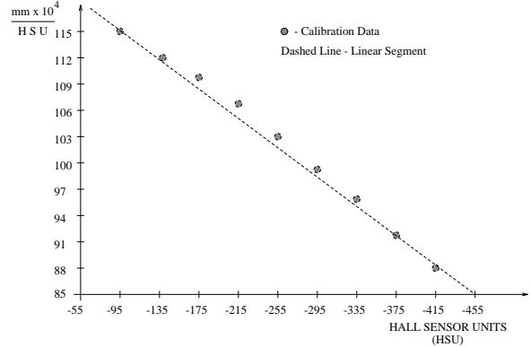
Figure 4: One linear segment of the calibration function showing a comparison between actual SPM position and the linear approximation
