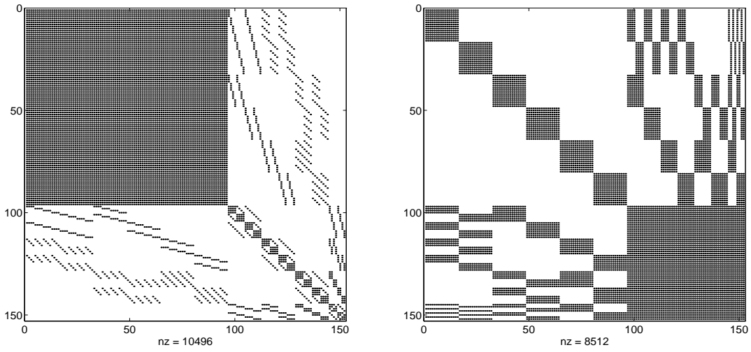
FIG. 5. Sparsity pattern of S^{(j)} (left) and of S_{J,Q}^{(j)} (right), for p = 5 , Method Q.
