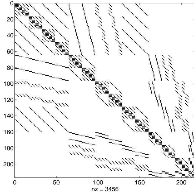
FIG. 4. Sparsity pattern of K^{(j)} , for p = 5 , Method Q.
