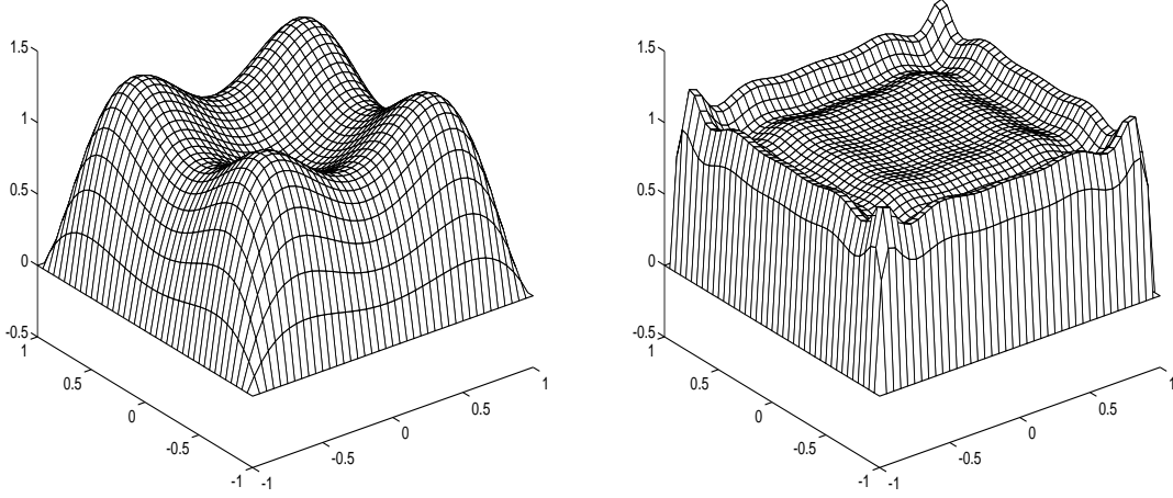
FIG. 3. \mathcal{F}_{Q,j} on a face of \Omega_{ref} , for p = 5 , and p = 10
