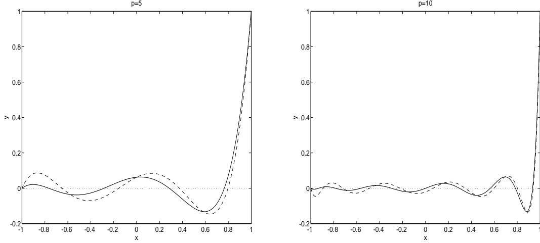
FIG. 2. l_0 (solid line) and \varphi_0 (dashed line) for p = 5 and p = 10
