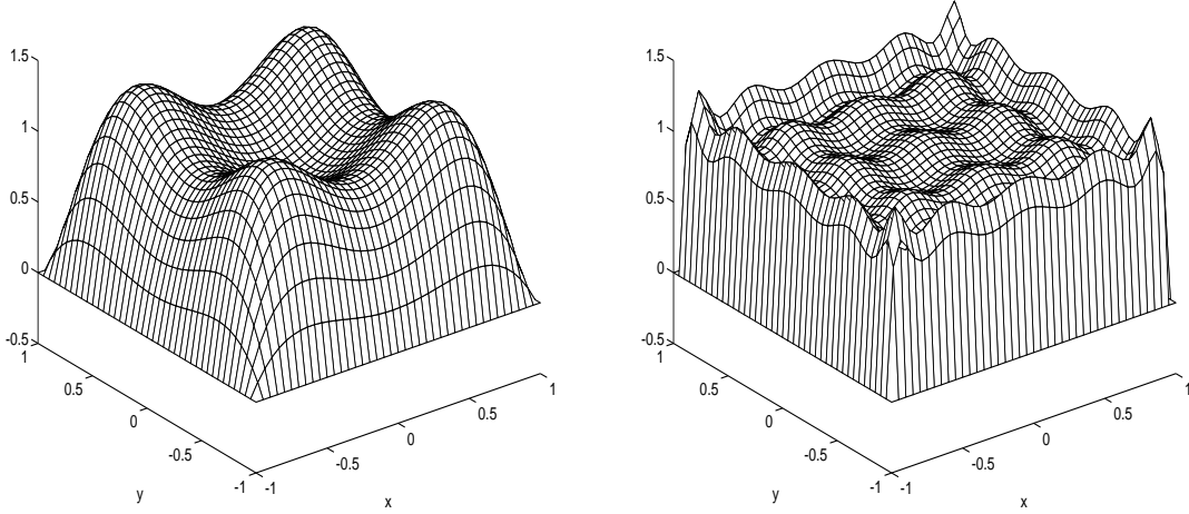
FIG. 1. \mathcal{F}_{G,j} on a face of \Omega_{ref} , for p = 5 , and p = 10
