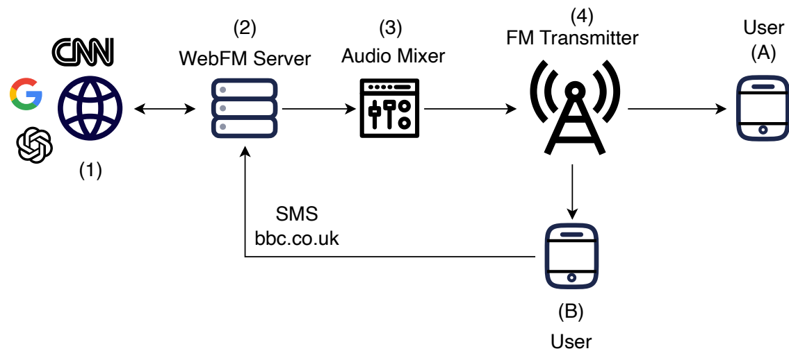
Figure 2.5: Sonic workflow.
