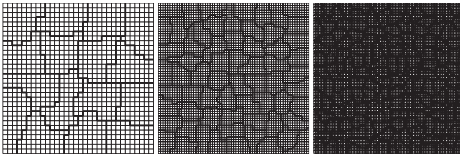
FIG. 4.2. Example decompositions obtained from a mesh partitioner.
