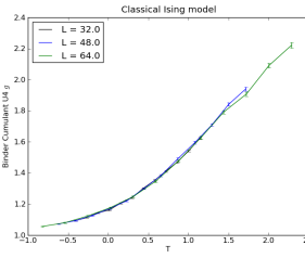
Figure 3. In this example we show a data collapse of the Binder Cumulant in the classical Ising model...
