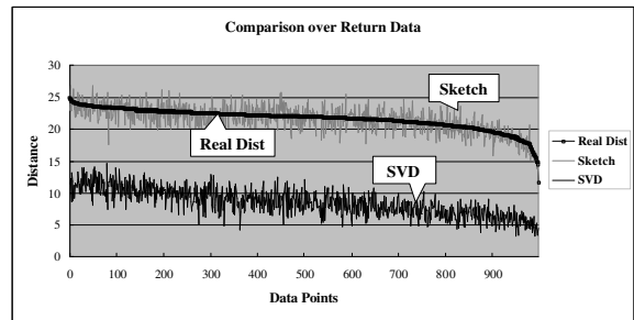
Figure 2: The sketch approach is superior to the Singular Value Decomposition, Wavelet, and Discrete Fourier Transform approaches for uncooperative time series. Of those three, Singular Value Decomposition is the best so is the one to which sketches are compared.
