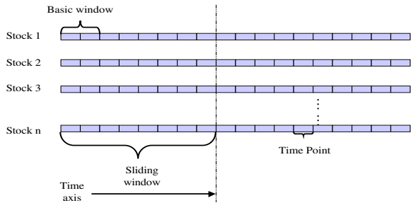
Figure 1: Sliding windows and basic windows.
