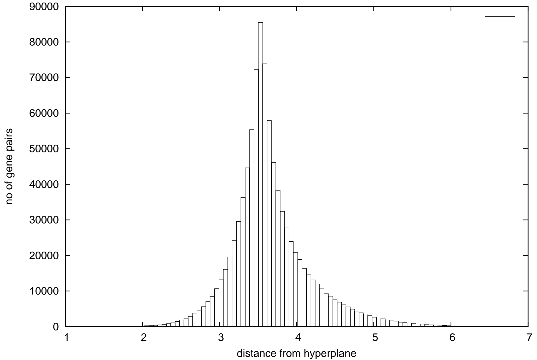
Frequency distribution - Trainingset 5 (part3)
