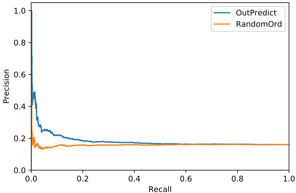
Precision-Recall Curves
