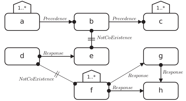
Fig. 5. An example of a DECLARE model.
