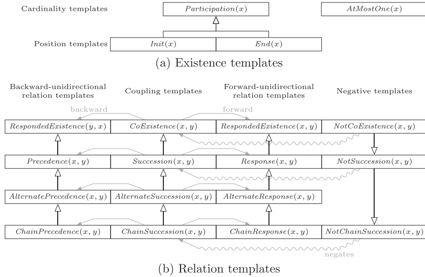
Fig. 1. The subsumption map of DECLARE templates. Templates are indicated by solid boxes. The subsumption relation is depicted as a line starting from the subsumed template and ending in the subsuming one, with an empty triangular arrow recalling the UML IS-A graphical notation. The coupling constraint templates are linked to the related forward-unidirectional relation constraint and backward-unidirectional relation constraint templates by means of grey arcs. The negative constraint templates are graphically linked to the corresponding coupling constraint templates by means of wavy grey arcs.
