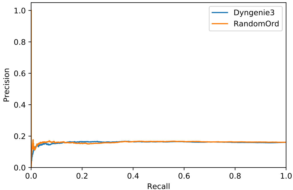
Precision-Recall Curves
