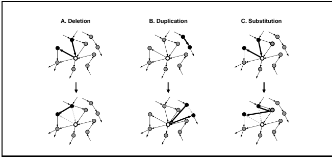
Figure 2: The three processes during graph evolution: deletion , duplication , and substitution . In each process, the target node (clear circle) is chosen with preference for nodes with larger degrees: if the i -th node has degree k_i , the probability of it being chosen is proportional to \frac{k_i}{\sum_{j=1}^N k_j} . In deletion ( A ), a pair of edges of the target node (thick black arrows), one incoming and one outgoing, is randomly chosen and deleted, and a new edge (thick black arrow) is added between the ascendent and descendent nodes (black filled circles). In duplication ( B ), new edges are added between the target node and the ascendent/descendent nodes (black filled circles) of an edge (thick black arrow) randomly chosen to be deleted. In substitution ( C ), a randomly chosen pair of edges of the target node (thick black arrows), one incoming and one outgoing, is rewired to a randomly chosen substitute node (gray filled circle with a thick boundary). Note that all the processes during graph evolution preserve the equality of the in-degree and out-degree of each node.
