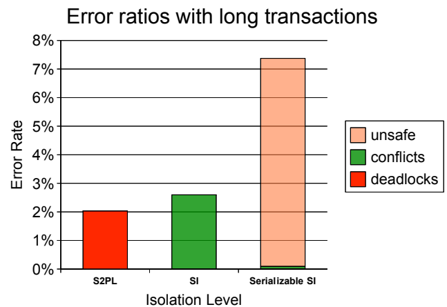
(b) Relative error rates of SI, S2PL and Serializable SI at MPL 20 with log flushes
