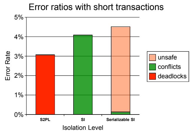
(b) Relative error rates of SI, S2PL and Serializable SI at MPL 20 without log flushes
