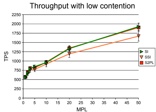
Figure 13: Throughput with low contention
