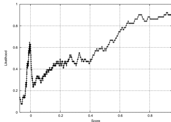
Figure 2: Correlation of the score and the likelihood of being a Named Entity (Single-word). The horizontal axis shows the score of a word. The vertical axis shows the likelihood of being a NE. One can see that the likelihood of NE increases as the score of a word goes up. However there is a huge peak near the score zero.
