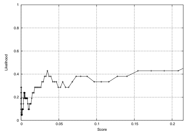
Figure 3: Correlation of the score and the likelihood of being a Named Entity (Multi-word). The horizontal axis shows the score of a word. The vertical axis shows the likelihood of being a NE.
