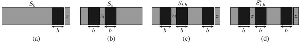
Figure 1: Illustration of the sequences derived from S that are considered in the proofs.
