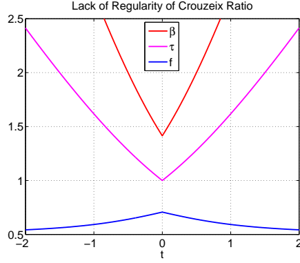
Fig. 1 Plot of the denominator \beta , the numerator \tau and the Crouzeix ratio f evaluated at (c, A + tA^2) , where c = [0, 1]^T (so p(\zeta) = \zeta ) and A is the 3 \times 3 Jordan block scaled by \sqrt{2} , for t \in [-2, 2] . This example shows that f is not regular at (c, A) .
