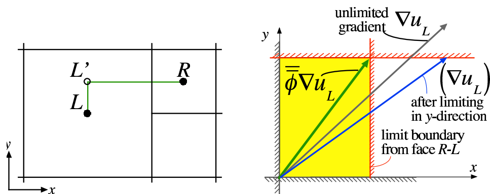
Figure 10. On the left is a typical mesh refinement interface in the x direction. On the right is its associated monotonicity polygon.
