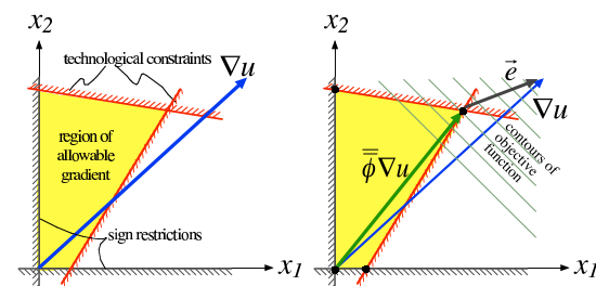
Figure 9. Directional limiting recast in LP framework. The limiter on each cell face imposes technological constraints as shown on the left. On the right, the final limited gradient is the optimal solution of the LP problem seeking minimize reduction of the gradient vector over the monotonicity region.
