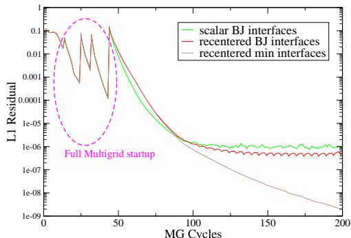
Figure 13. Convergence in the L1 norm of the density residual subsonic OneraM6 wing example ( M_\infty = 0.5 , \alpha = 3.06^\circ ).
