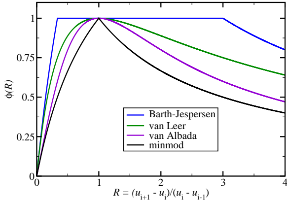
Figure 2. Common limiters in slope form from (8).
